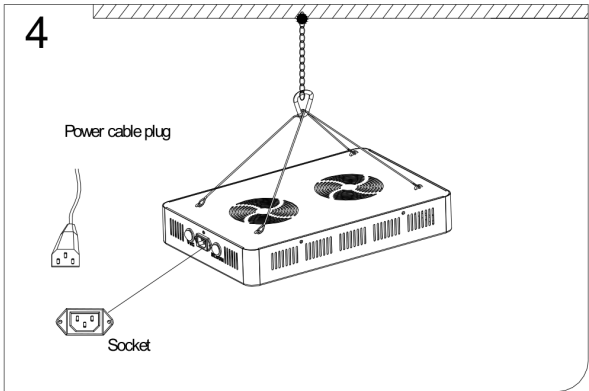
4. Match the power cable plug with socket, finally turn on the power to test luminaires.
